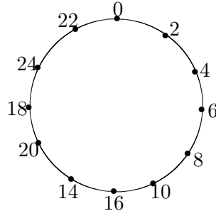
Figure 4: An even vertex odd mean labeling of C_{12}
